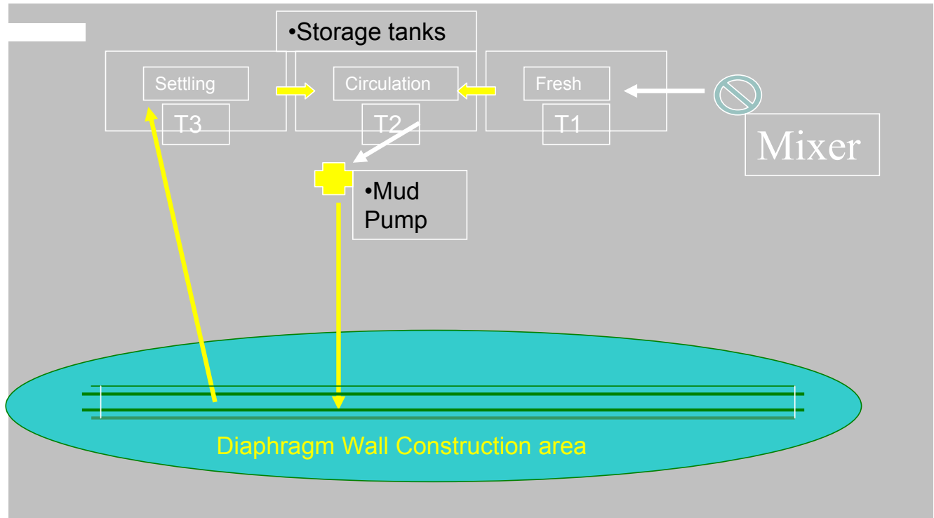
Schematic Diagram of Bentonite Setup
